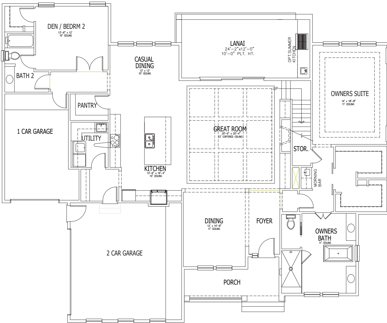
FIRST FLOOR
